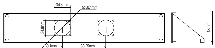
▲ 2 RU panel for 2 × Burndy B48 type connectors
