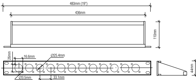
▲ 1 RU panel for 12 × AXR 31/34 type connectors
