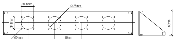
▲ 2 RU panel for 4 × Burndy B48 type connectors
