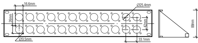
▲ 2 RU panel for 24 × AXR 31/34 type connectors
