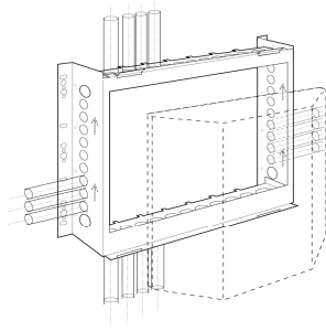
▲ Mounted over surface conduit
