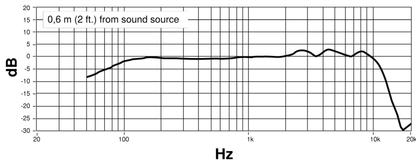
Frequency Response
