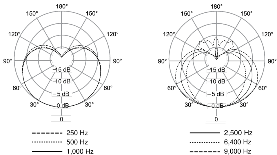
Polar Pattern
